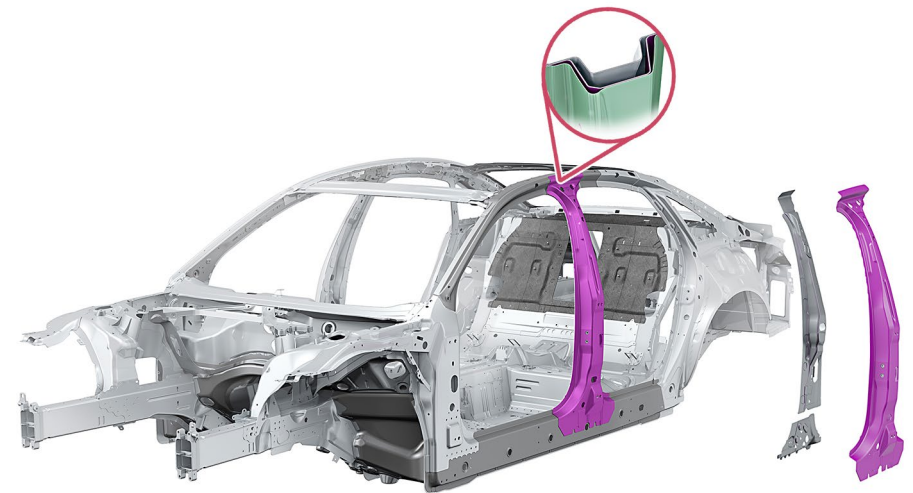
B-pillar with multi-shell structure
