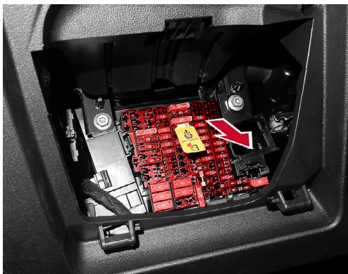
Emergency cut-out connection, fuse carrier
