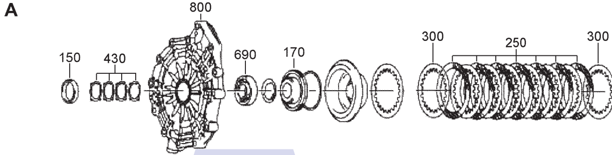
Front Cover & Forward Clutch
