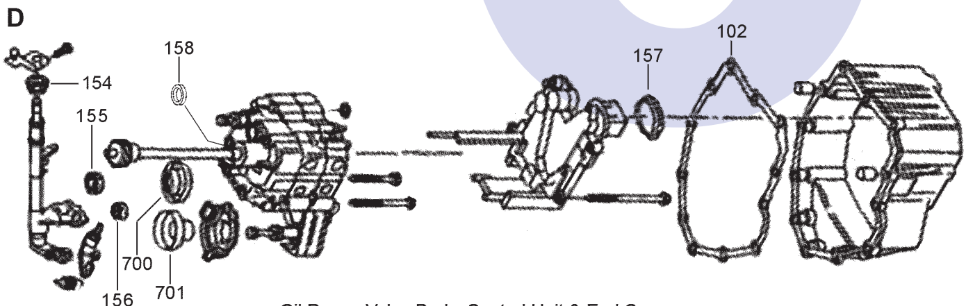
Oil Pump, Valve Body, Control Unit & End Cover
