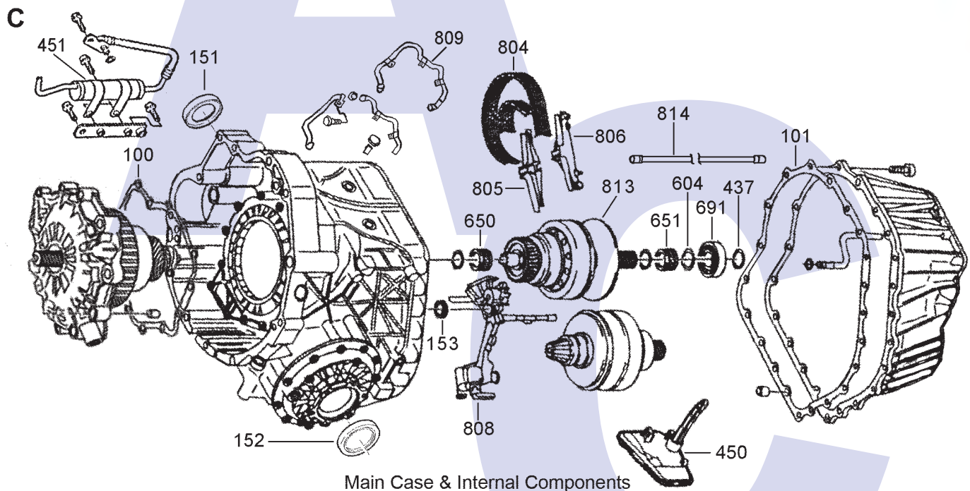
Forward Clutch Drum & Reverse Brake
