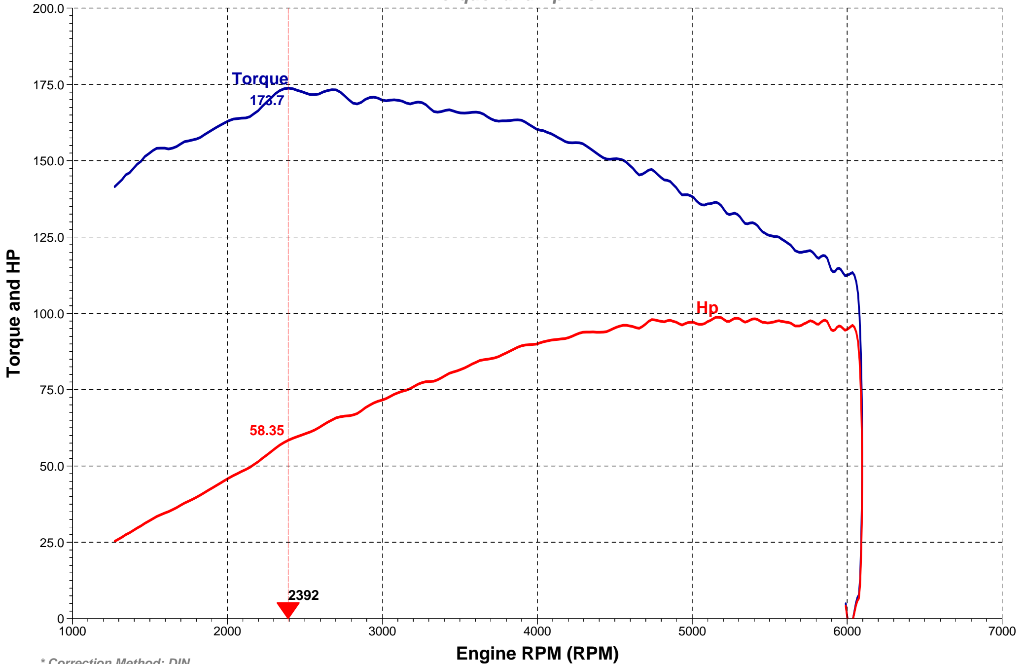
Torque* and Hp* vs. RPM
